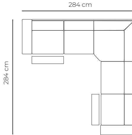
2.5 seat small square corner modular with 2 recliners
